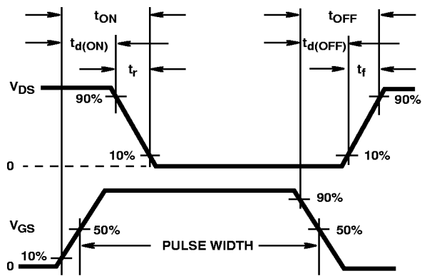
FIGURE 17. SWITCHING WAVEFORMS
