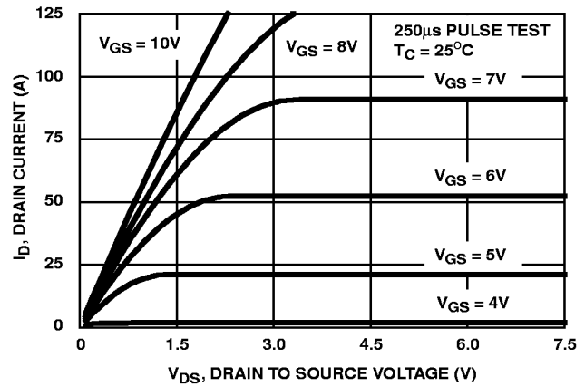
FIGURE 7. SATURATION CHARACTERISTICS
