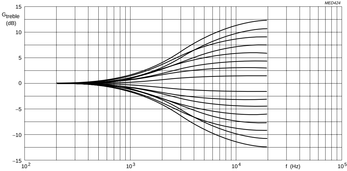
Fig.4 Treble control.
