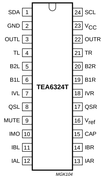
Fig.2 Pin configuration.
