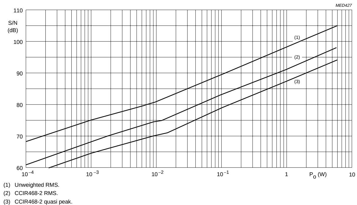
Fig.6 Signal-to-noise ratio; V_i = 2 \text{ V} ; P_{\max} = 6 \text{ W} .
