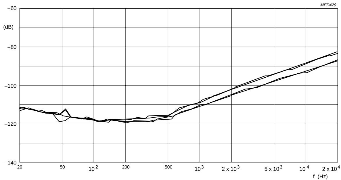
Fig.8 Muting.
