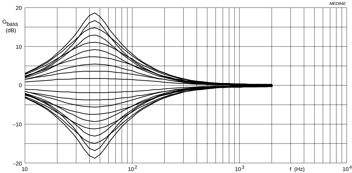
Fig.3 Bass control.
