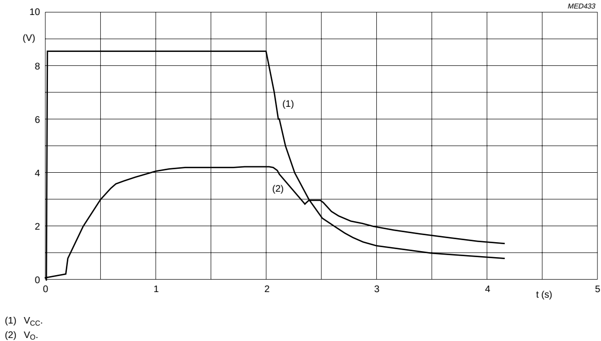
Fig.12 Turn-on/off behaviour.
