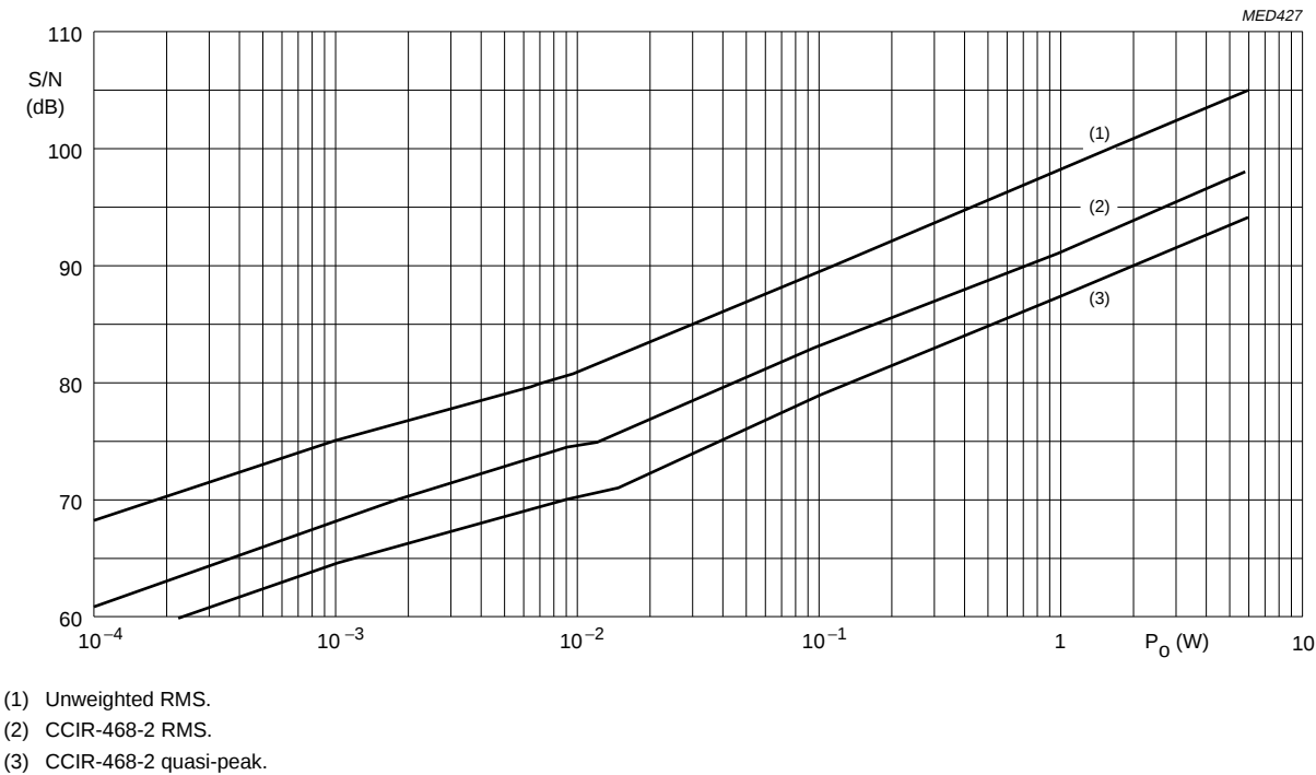
Fig.7 Signal-to-noise ratio; V_i = 2\text{ V} ; P_{\text{max}} = 6\text{ W} .
