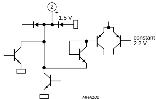
Fig.25 Pin 2: mute control.
