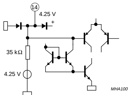
Fig.24 Pins 14, 16 to 18, 20, 21, 23, 25, 27: inputs.
