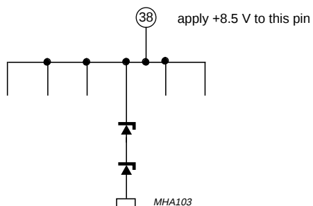
Fig.27 Pin 38: supply voltage.
