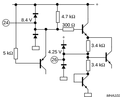
Fig.26 Pin 24: filtering for supply; pin 26: reference voltage.
