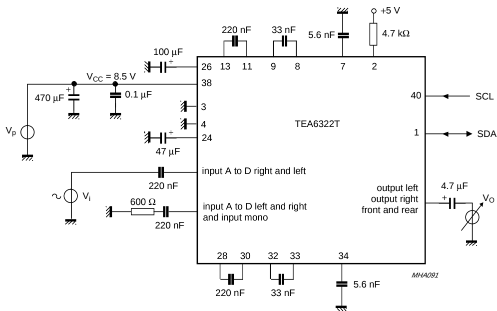
Fig.14 Test circuit for channel separation ( \alpha_{CS} ).
