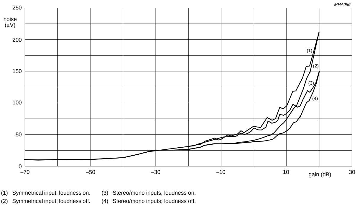
Fig.8 Noise output voltage; CCIR468-2, quasi peak.
