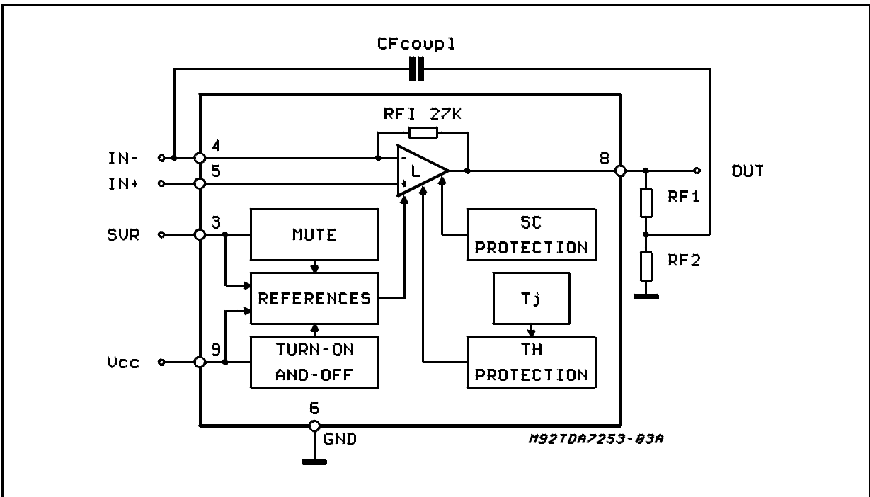
Figure 1: Application Circuit
