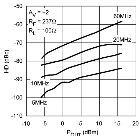
HD2 vs. Output Power (across 100Ω) (SOIC package)
