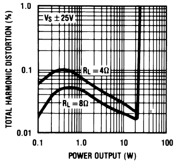
THD vs Power Output
