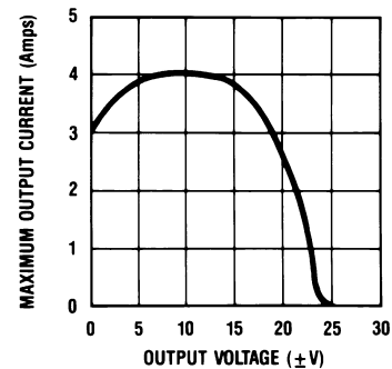
Current Limit vs Output Voltage*
