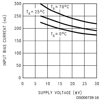
I_B vs Supply Voltage
