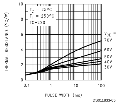
Pulse Thermal Resistance
