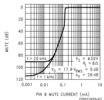
Mute Attenuation vs Mute Current
