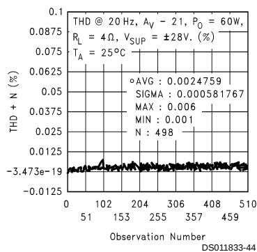
THD + N Distribution
