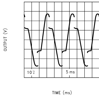
SPiKe Protection Response
