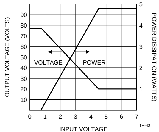
FIGURE 2. CVA2417TX DC Characteristics
